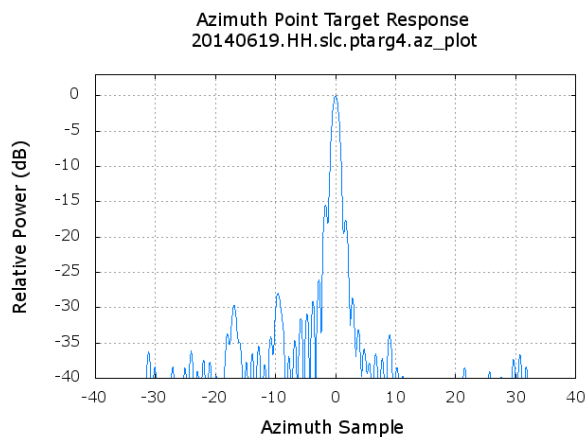
Figure 5 Point target response in azimuth.
